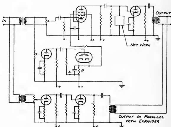
FIG. 5. Linear-non-linear combination.
